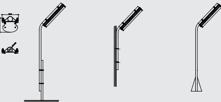
Pole Mounting
