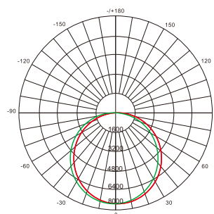
CP06-240L-57
