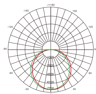
CP06-180L-57
